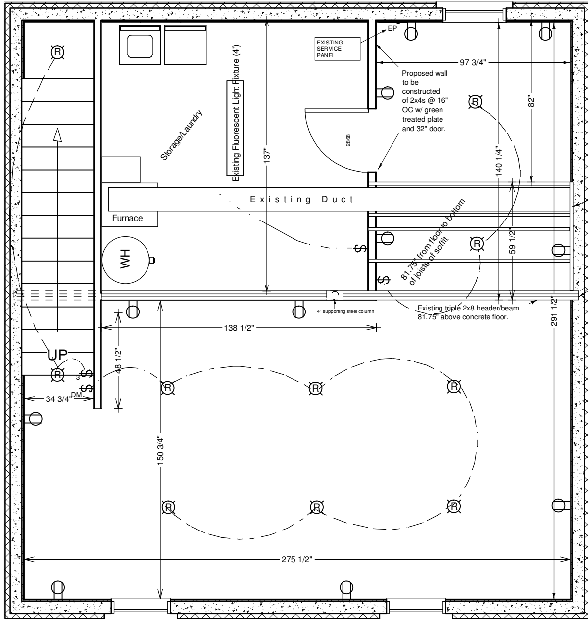
LIVING AREA 616 sq ft
